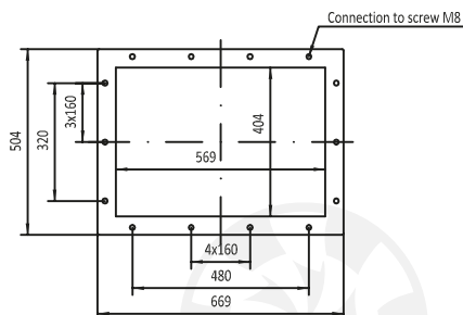
OUTLET FLANGE DETAIL
