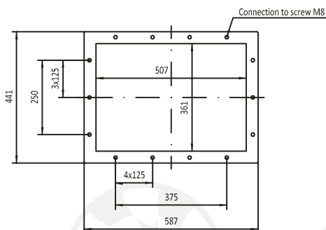
OUTLET FLANGE DETAIL
